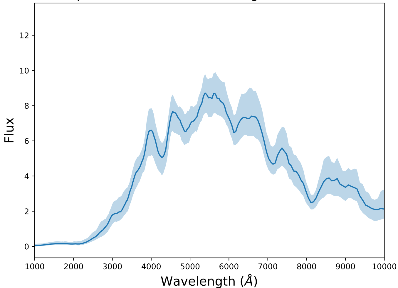
Spectrum 1 for transient 91bg-like at z=1.23
